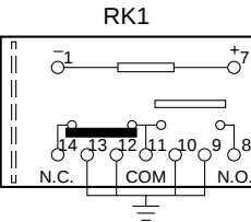
Standard contact arrangement
