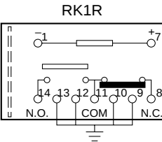
R type contact arrangement
