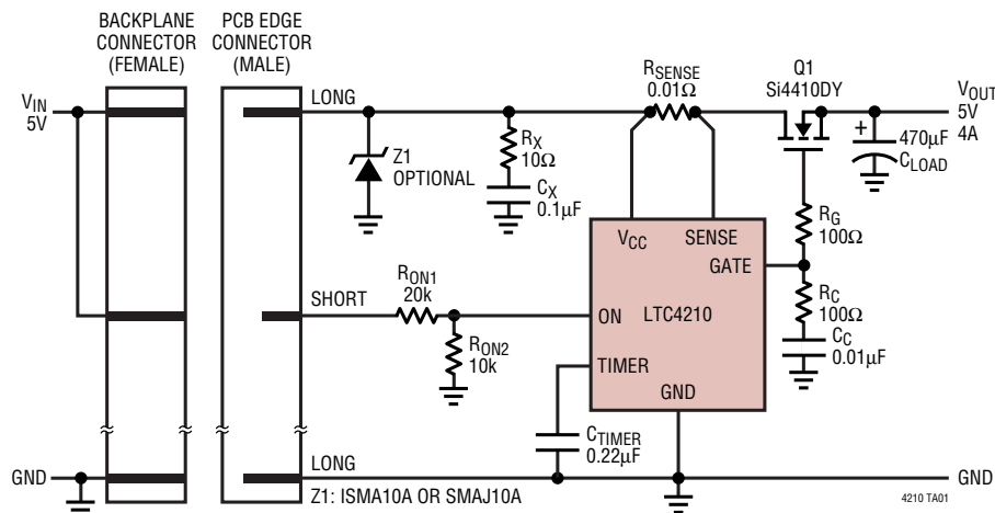
Single Channel 5V Hot Swap Controller
