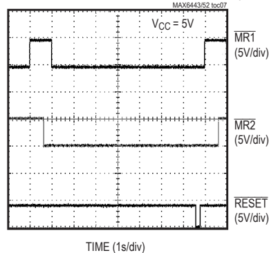
MANUAL RESET TO RESET DELAY (MAX6445L/MAX6446L/MAX6449L/MAX6450L)
