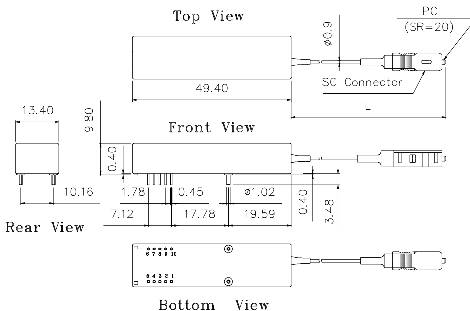
BTRS-9780-1590-SP50G
