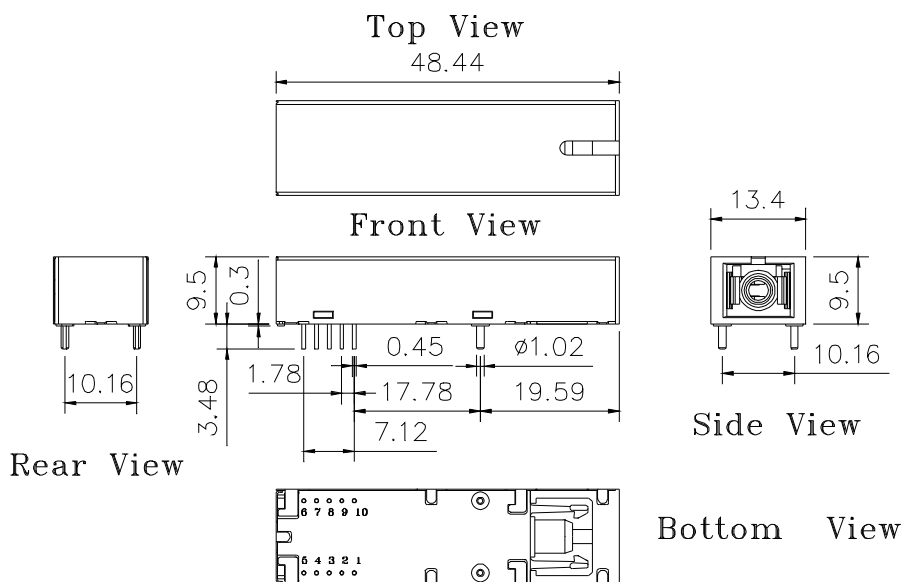
BTRS-9780-1590G
