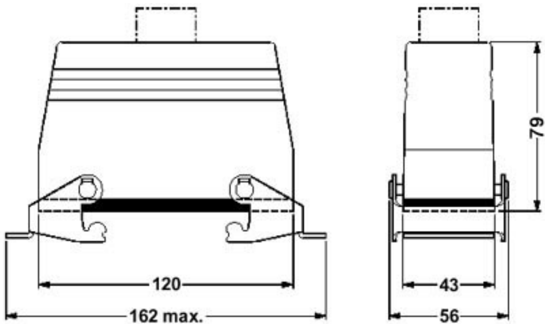
Dimensioned drawing
