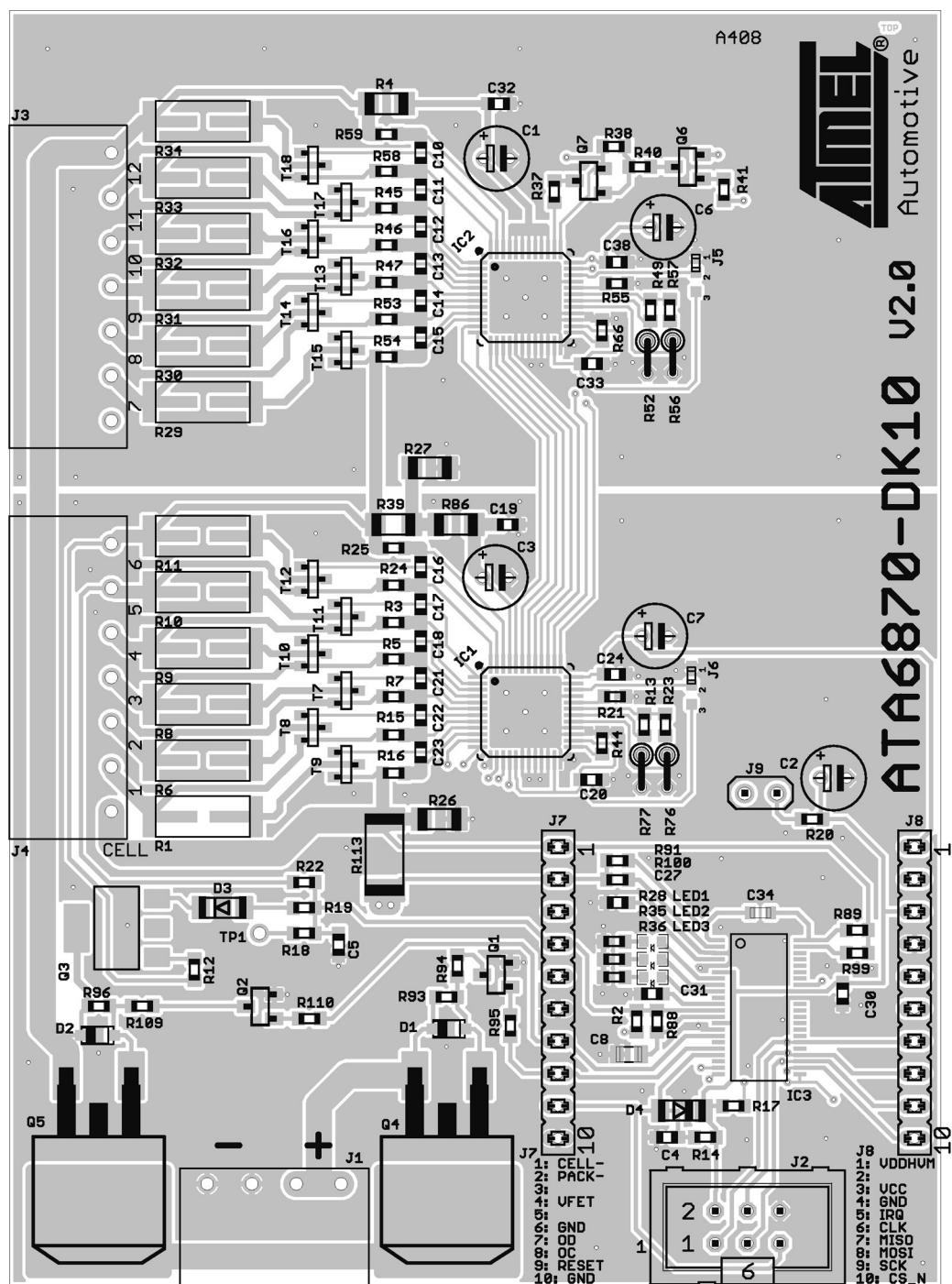
Figure 7-2. PCB Top
