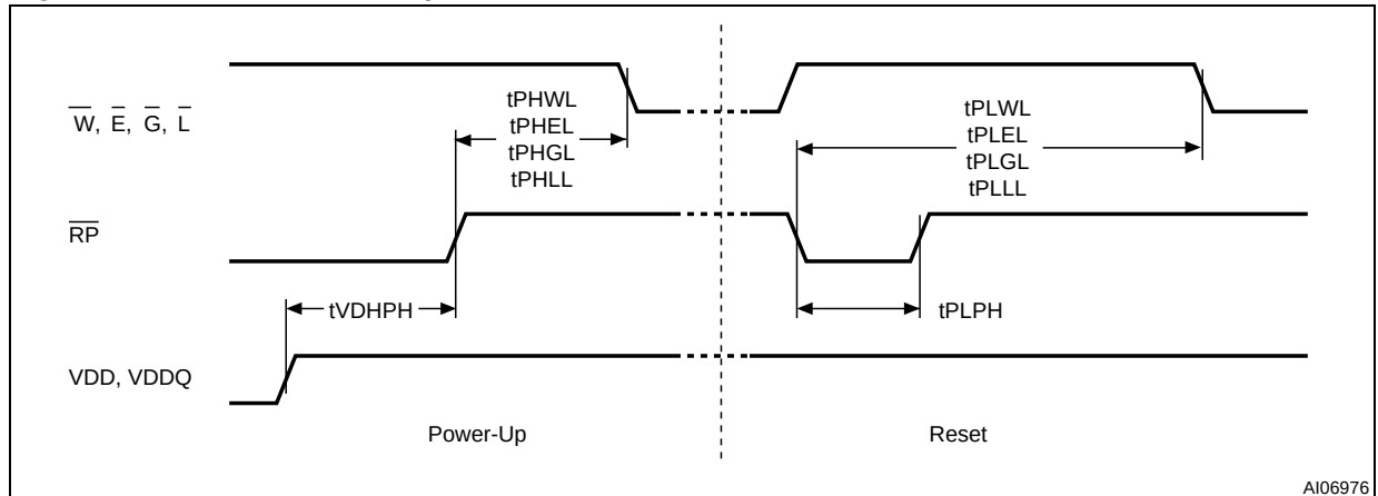
Figure 18. Reset and Power-up AC Waveforms
