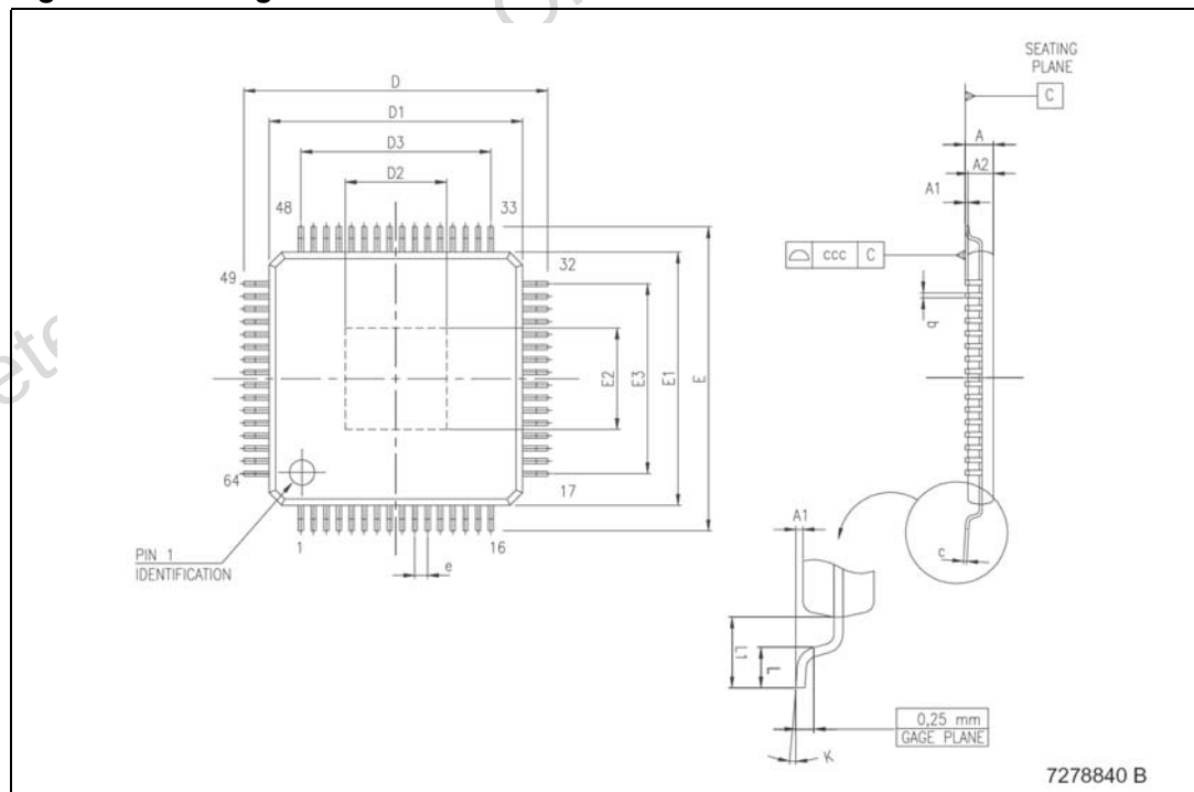
Figure 27. Package dimensions
