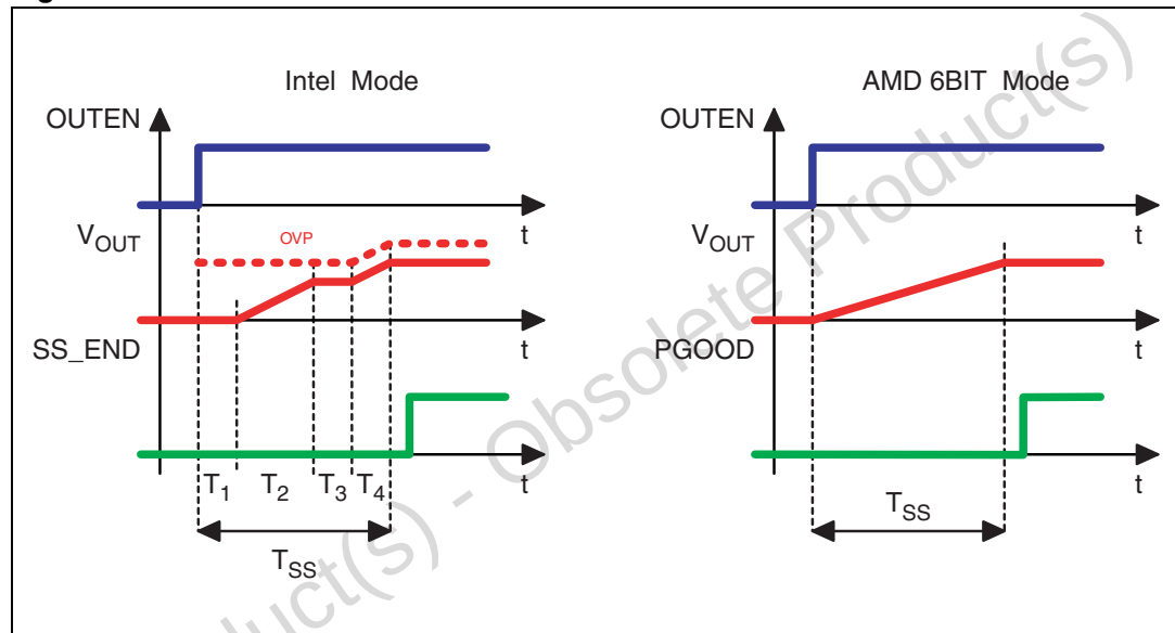
Figure 14. Soft start
