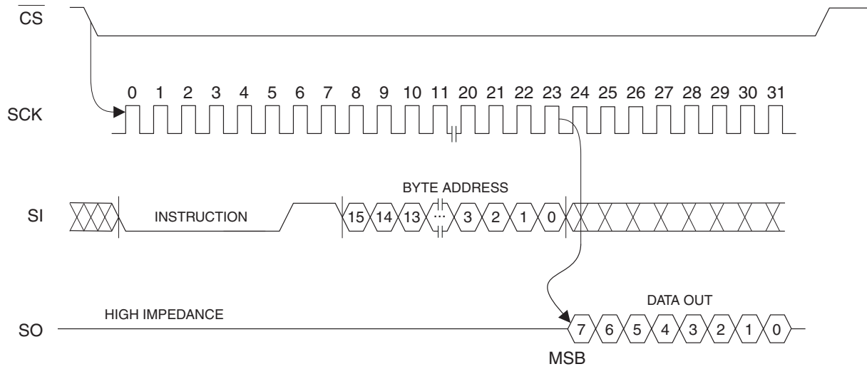
Figure 4-6. READ Timing
