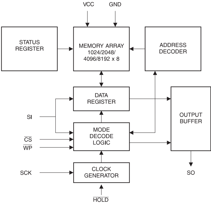
Figure 1-1. Block Diagram
