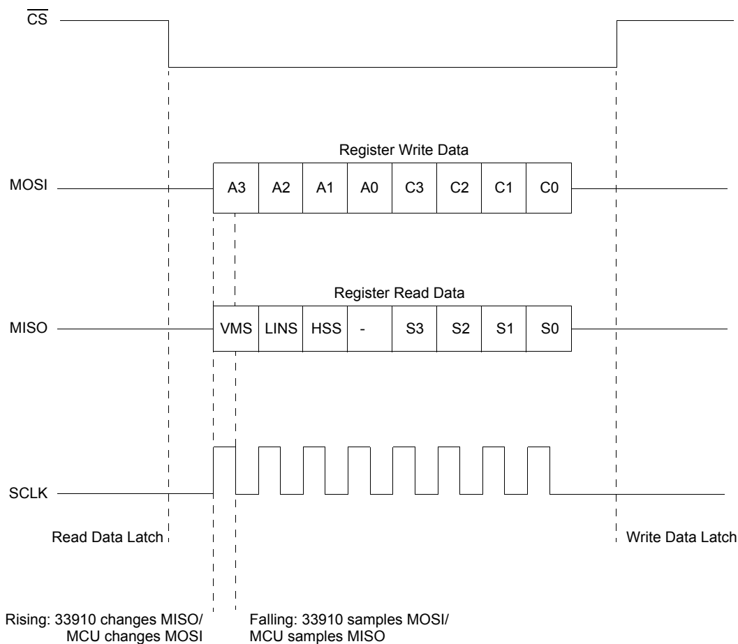
Figure 19. SPI Protocol
