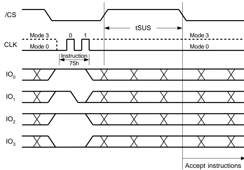
Figure 35b. Erase/Program Suspend Instruction (QPI Mode)
