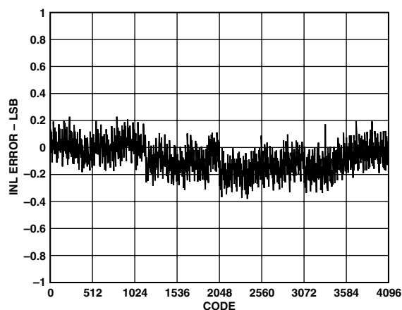
Figure 18. Typical INL for 2.75 V @ +25°C
