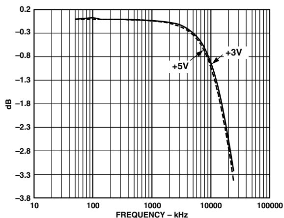
Figure 24. Typical Bandwidth
