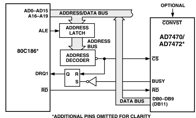
Figure 30. Interfacing to the 80C186
