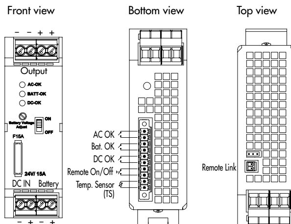
Connector Positions
