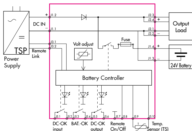
Function Diagram
