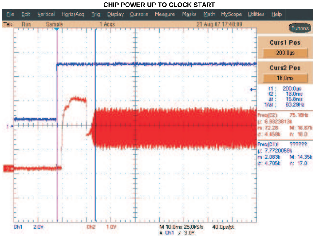
Figure 5-1. Power Up [ V_{IN} (Blue) to Crystal Start (Red)]
