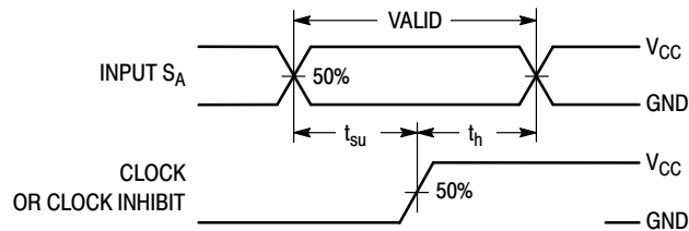
Figure 5. Serial-Shift Mode
