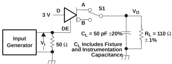
Figure 6. Driver High-Level Enable and Disable Time Test Circuit and Voltage Waveforms
