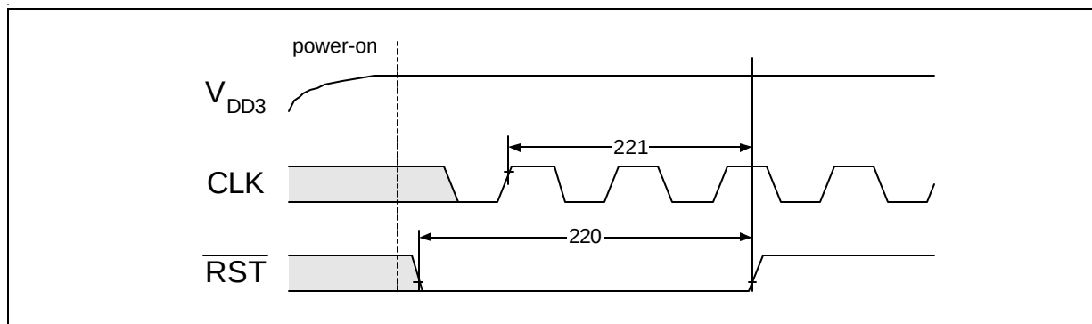
Figure 9-26 Reset Timing
