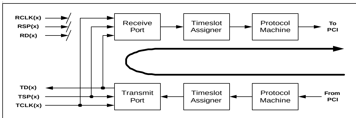
Figure 4-2 Local Port Loop
