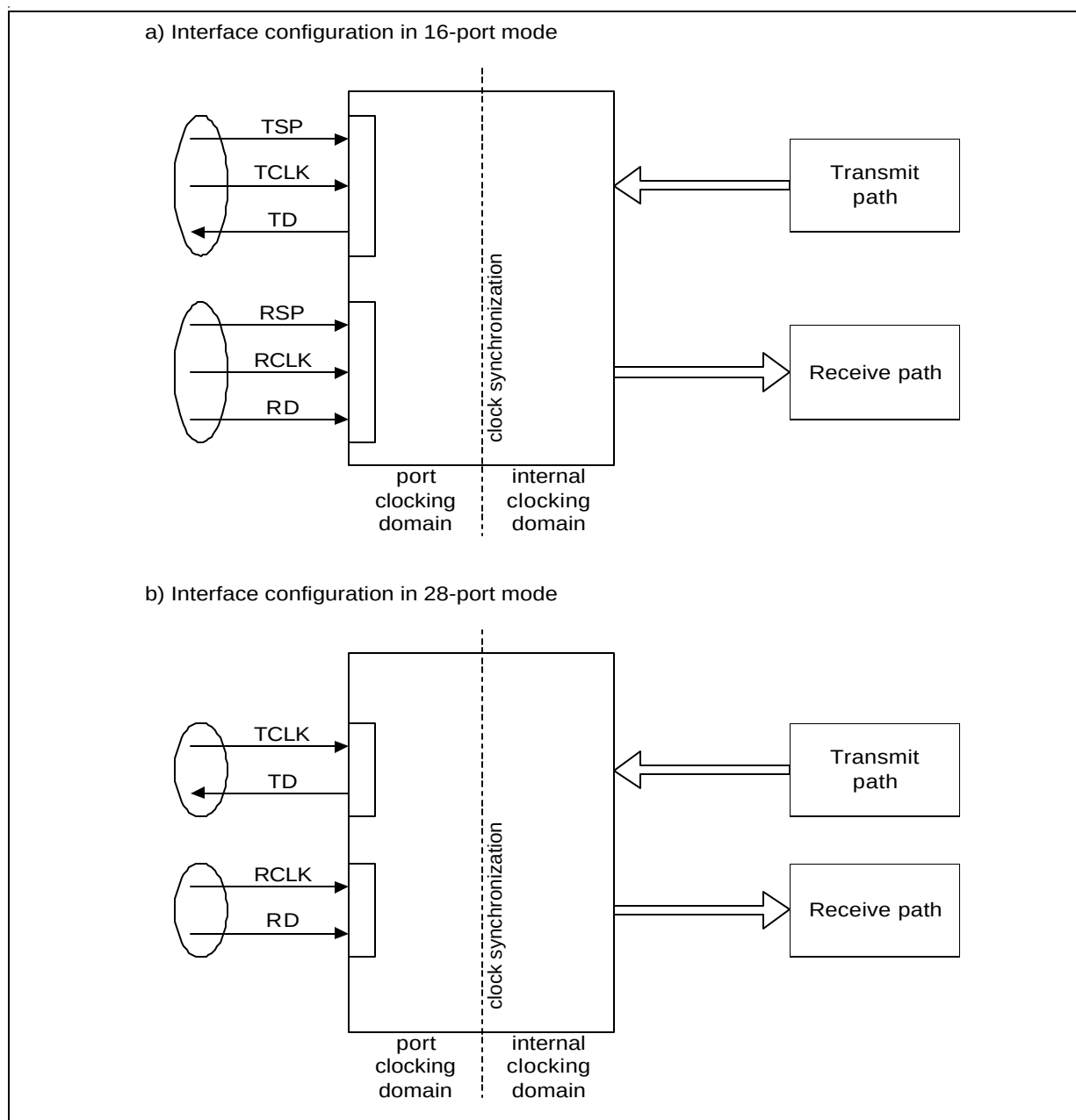
Figure 4-1 Port Configuration
