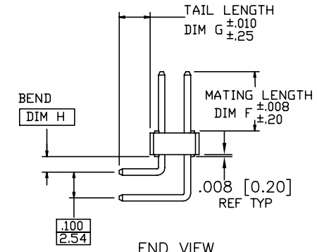
END VIEW
