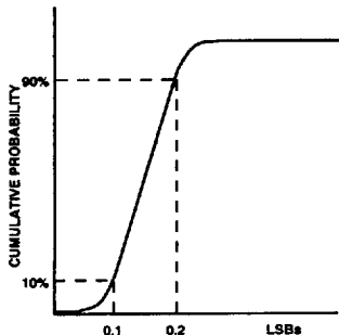
Figure 3. INL Statistics
