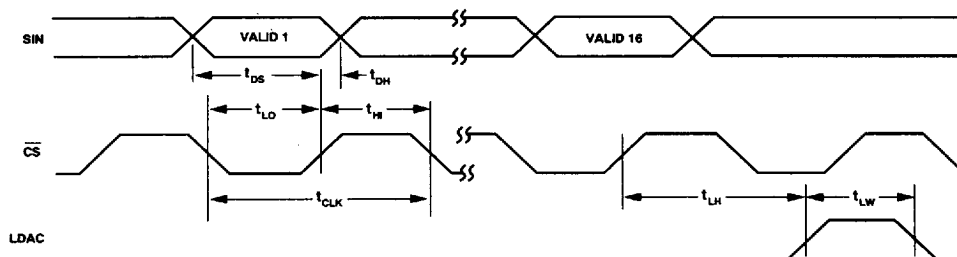
Figure 1b. AD760 Serial Load Timing
