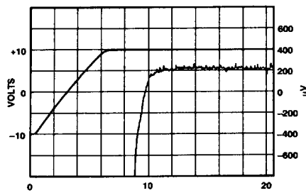
a. -10 V to +10 V Full-Scale Step Settling
