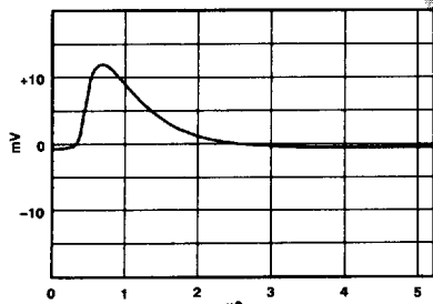
c. D-to-A Glitch Impulse
