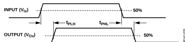
Figure 28. Propagation Delay Parameters
