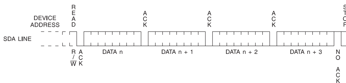
Figure 7-6. Sequential Read
