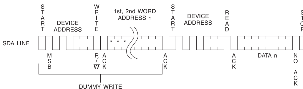
Figure 7-5. Random Read
