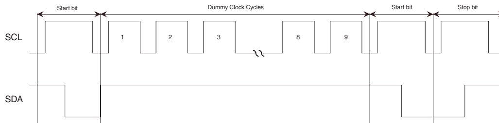
Figure 4-1. Software Reset
