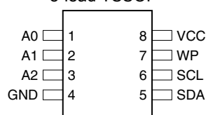
8-lead TSSOP
