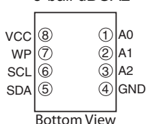
8-ball dBG2
