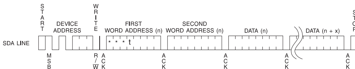
Figure 7-3. Page Write
