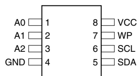
8-lead TSSOP
