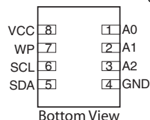
8-lead Ultra Thin Mini-MAP (MLP 2x3)
