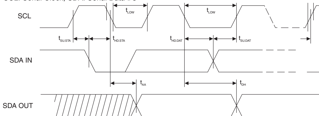
Figure 4-2. Bus Timing SCL: Serial Clock, SDA: Serial Data I/O
