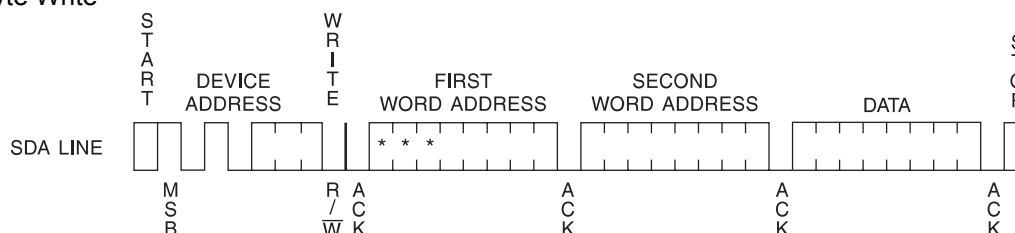
Figure 7-2. Byte Write
