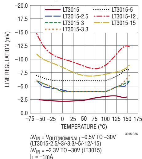
Line Regulation
