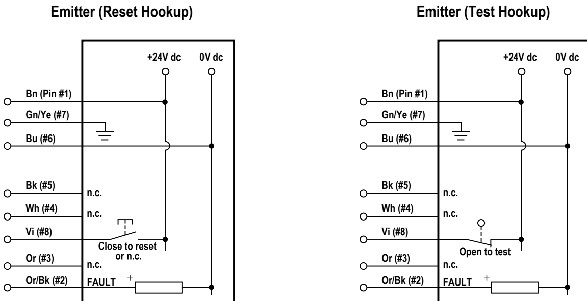
Figure 28. Emitter—Generic wiring
