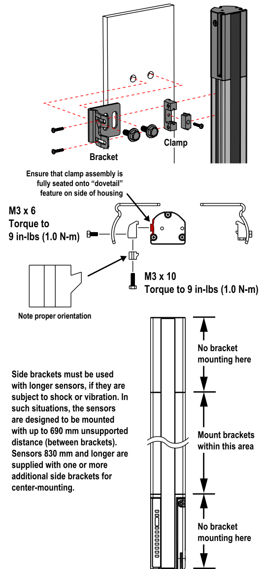
Figure 17. Side-mount hardware attachment
