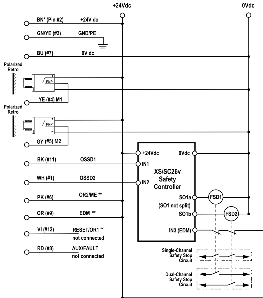
Figure 31. Generic wiring to a self-checking safety module, Safety Controller, safety PLC (no EDM, auto reset, no Override)
