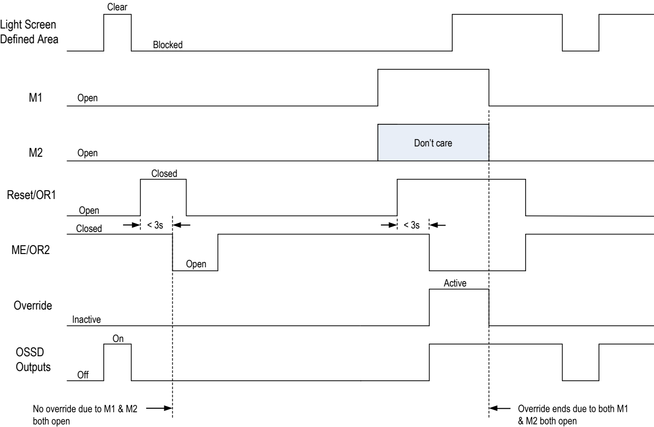
Figure 44. Timing logic: Mute configuration 5 or 6, Mute-Dependent Override Function
