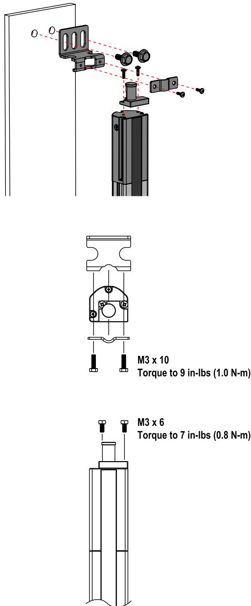
Figure 16. End-mount hardware attachment
