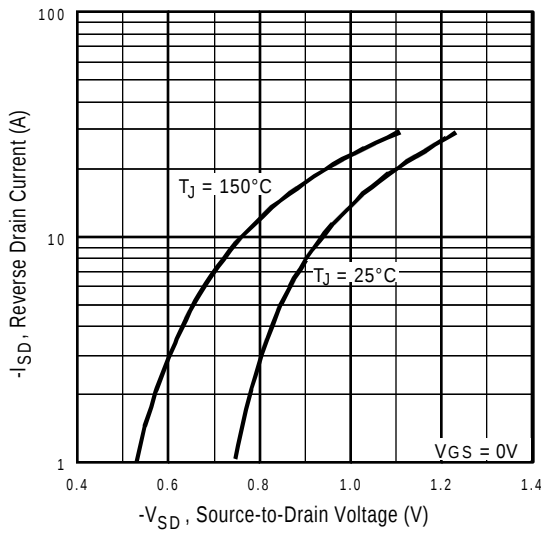
Fig 15. Typical Source-Drain Diode Forward Voltage
