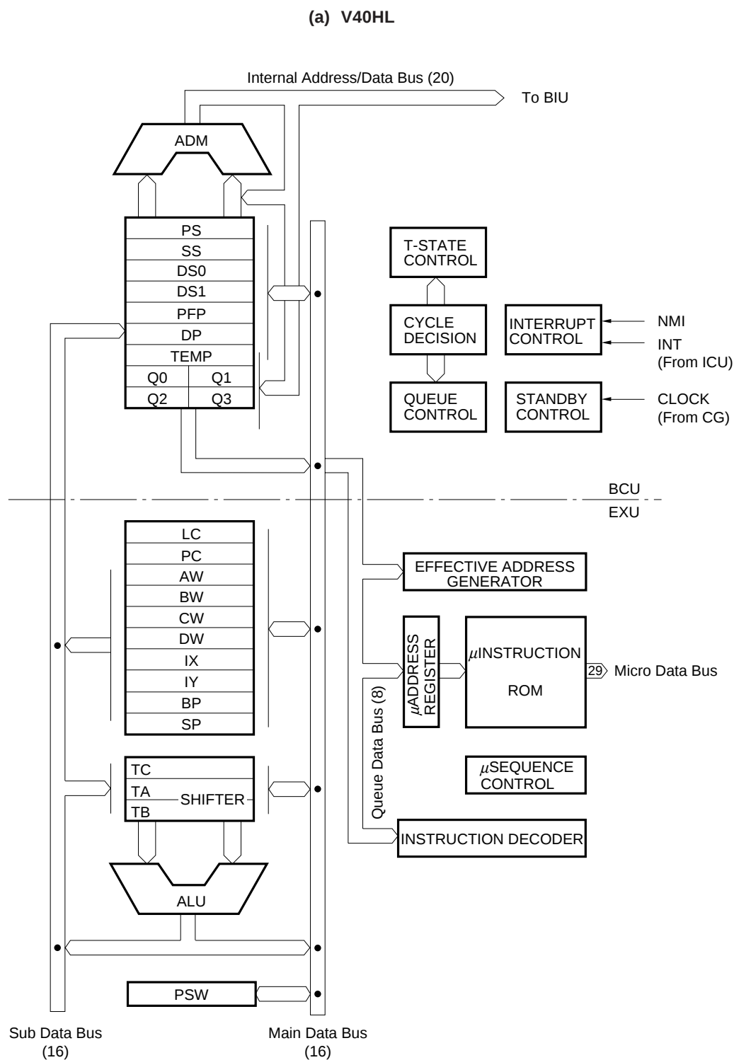
Figure 3-1. Internal Block Diagram of CPU (1/2)
