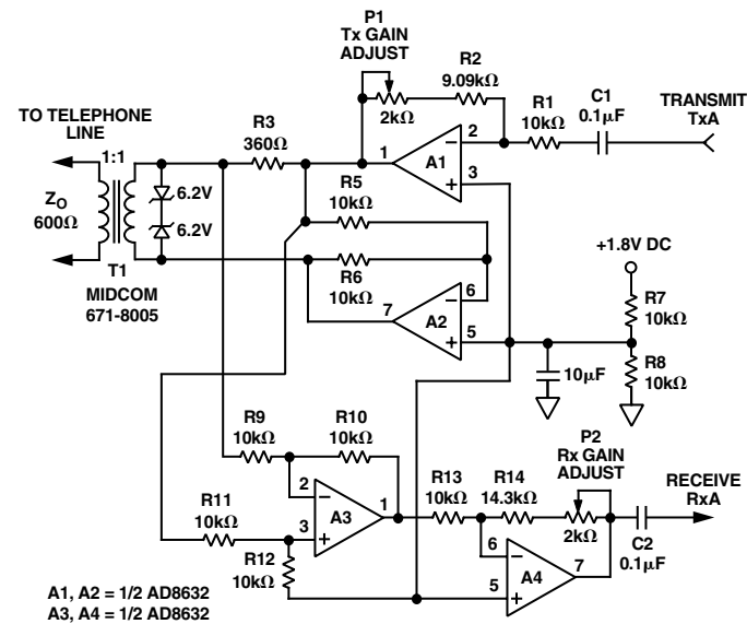
Figure 31. A Single-Supply Direct Access Arrangement for Modems
