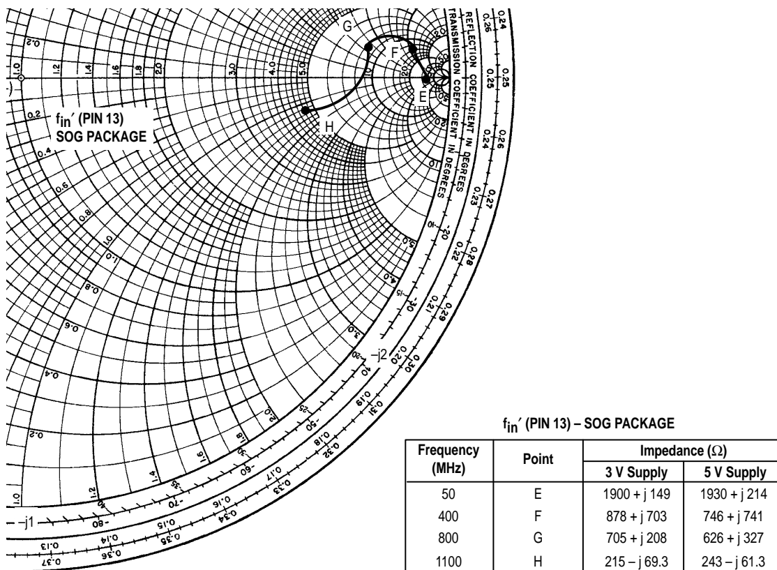
Figure 13. Nominal Input Impedance of f_{in} and f_{in'} — Series Format ( R + jX ) (50 – 1100 MHz)
