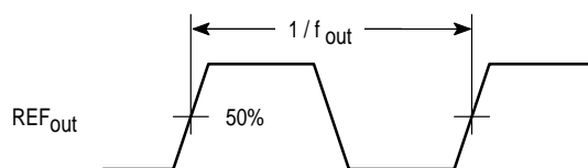
Figure 10. Switching Waveform
