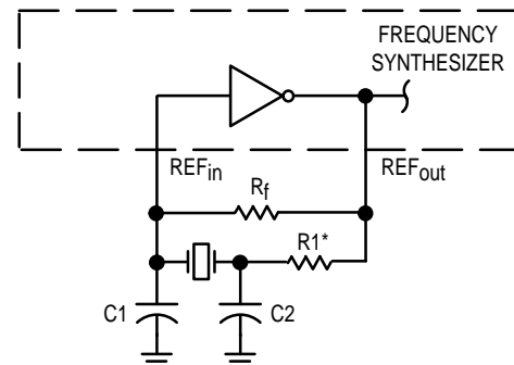
Figure 18. Pierce Crystal Oscillator Circuit
