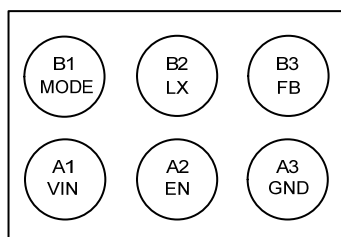
Figure 2. Pin Configuration(s)
