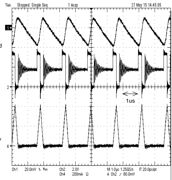
Figure 10. PFM mode Operation I_{out}=50\text{mA}
