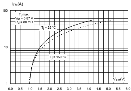
Figure 9. On-state characteristics (maximum values)
