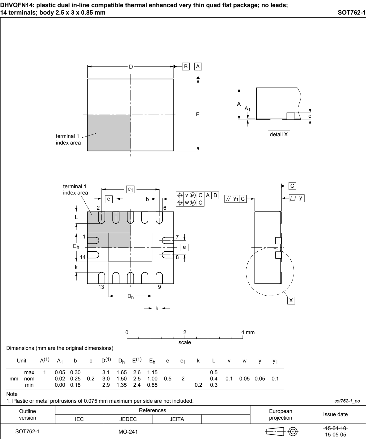
Figure 10. Package outline SOT762-1 (DHVQFN14)
