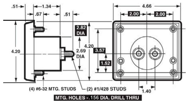
4-1/2" Models 2124, 2124T, 2144, 2154, 2184
