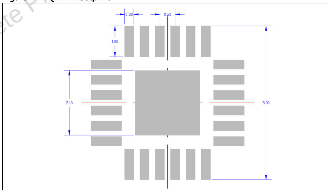
Figure 27. QFN24 footprint
