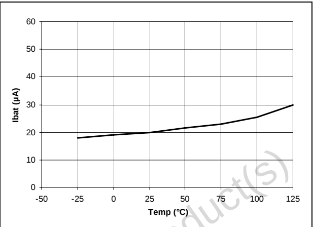
Figure 9. Battery standby current vs temperature (no MAIN, no USBPWR, gas gauge disabled)
