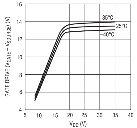
Gate Drive vs V_{\text{DD}}
