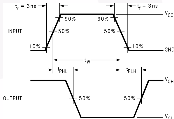
Figure 3. AC Waveforms
