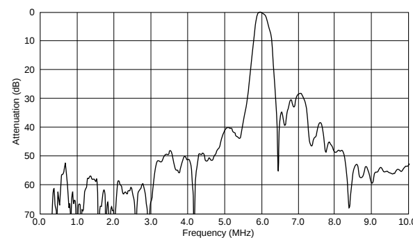
SFSRA6M00DF00-B0
