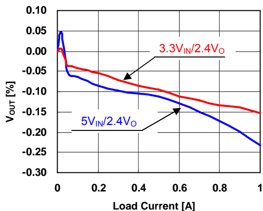
Figure 10. Normalized V_{OUT} vs. Load Current
