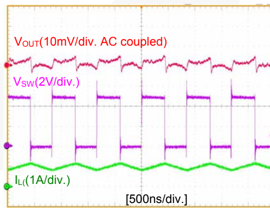
Figure 9. Output Voltage Ripple with 1A Load
