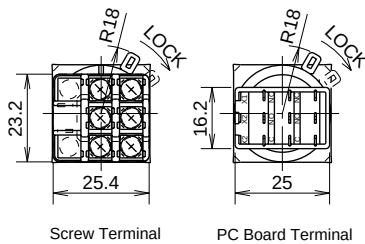
Screw Terminal
