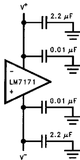
FIGURE 2. Power Supply Bypassing
