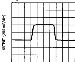
Small Signal Pulse Response A_V = +2 , V_S = \pm 15V
