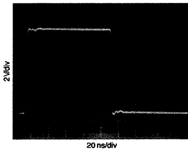
FIGURE 3. Properly Terminated Signal
