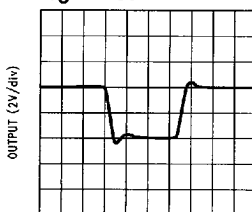
Large Signal Pulse Response A_V = -1 , V_S = \pm 5V
