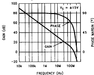
Open Loop Frequency Response
