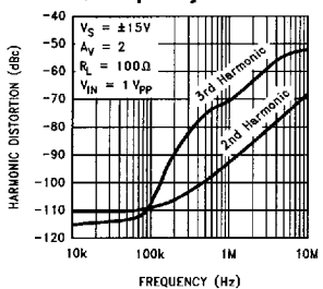
Harmonic Distortion vs Frequency
