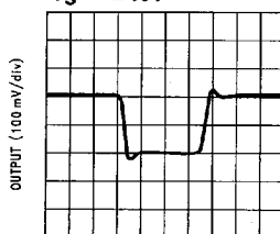
Small Signal Pulse Response A_V = -1 , V_S = \pm 15V
