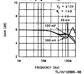
Closed Loop Frequency Response vs Input Signal Level ( A_V = +2 )
