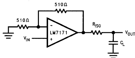
FIGURE 5. Isolation Resistor Used to Drive Capacitive Load
