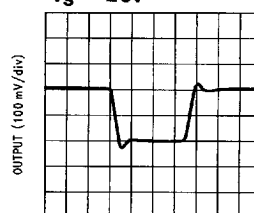
Small Signal Pulse Response A_V = -1 , V_S = \pm 5V
