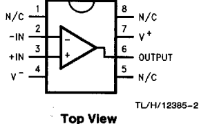
8-Pin DIP/SO
