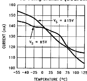
Short Circuit Current vs Temperature (Sourcing)
