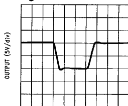
Large Signal Pulse Response A_V = -1 , V_S = \pm 15V
