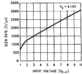
Slew Rate vs Input Voltage
