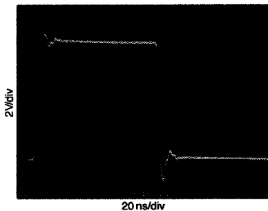
FIGURE 4. Improperly Terminated Signal
