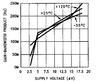
Gain-Bandwidth Product vs Supply Voltage
