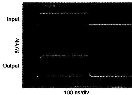
FIGURE 6. The LM7171 Driving a 150 pF Load with a 50 \Omega Isolation Resistor
