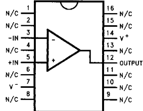
16-Pin Wide Body SO
