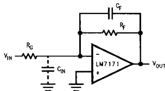
FIGURE 1. Compensating for Input Capacitance
