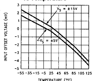
Input Offset Voltage vs Temperature
