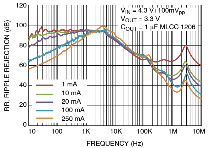
Figure 30. Power Supply Rejection Ratio – V_{\text{OUT}} = 3.3 \text{ V}
