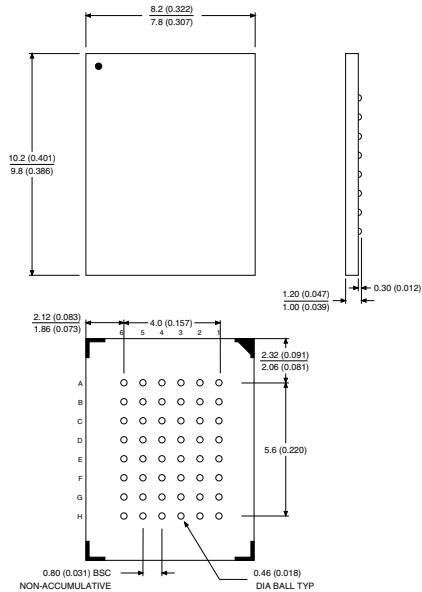
48U , 48-ball, Micro Ball Grid Array Package (µBGA) Dimensions in Millimeters
