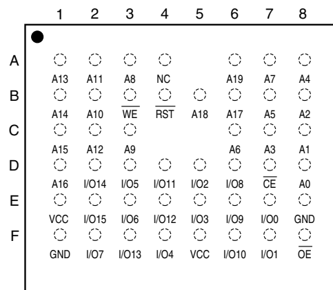
µBGA Top View (Ball Down)
