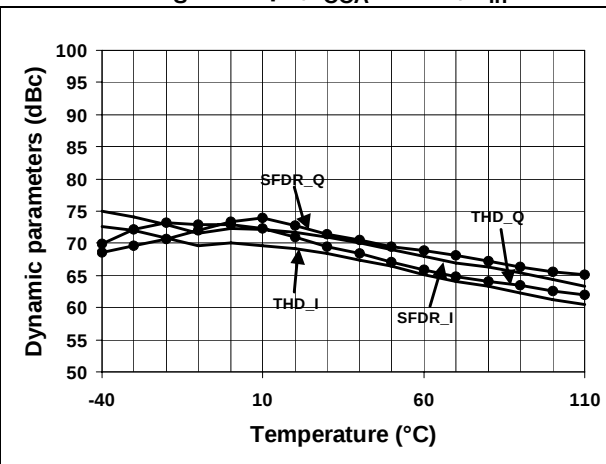
Figure 10. Distortion vs. temperature F_S = 40\text{Mps} , I_{CCA} = 60\text{mA} , F_{in} = 2\text{MHz}
