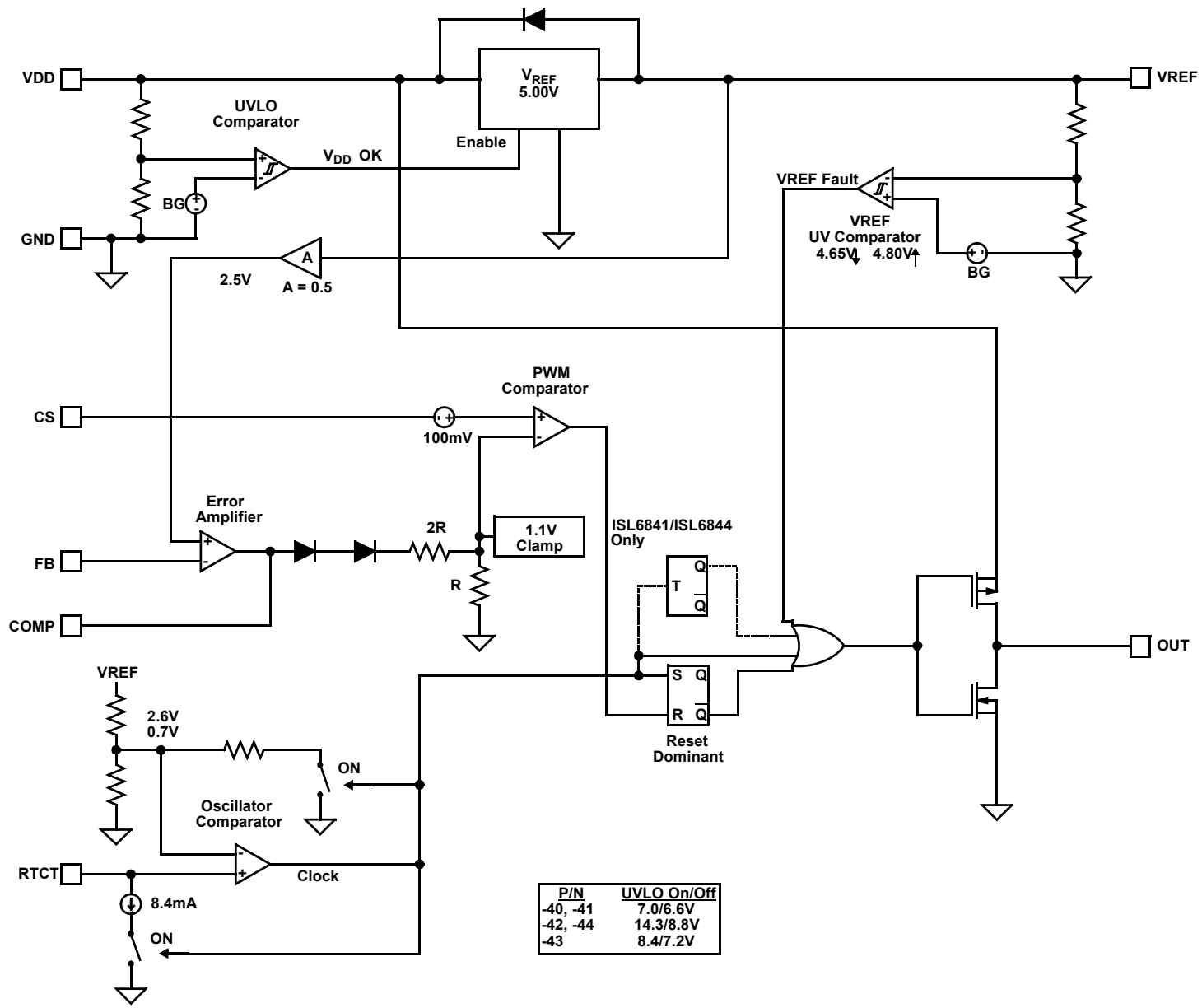
Figure 3. Block Diagram
