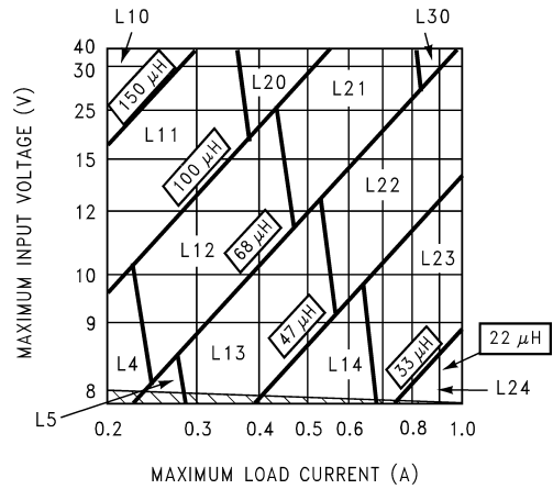
FIGURE 5. LM2675-5.0
