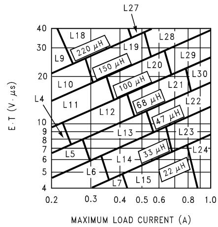
FIGURE 7. LM2675-ADJ
