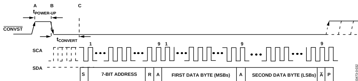
Figure 32. Mode 1 Operation
