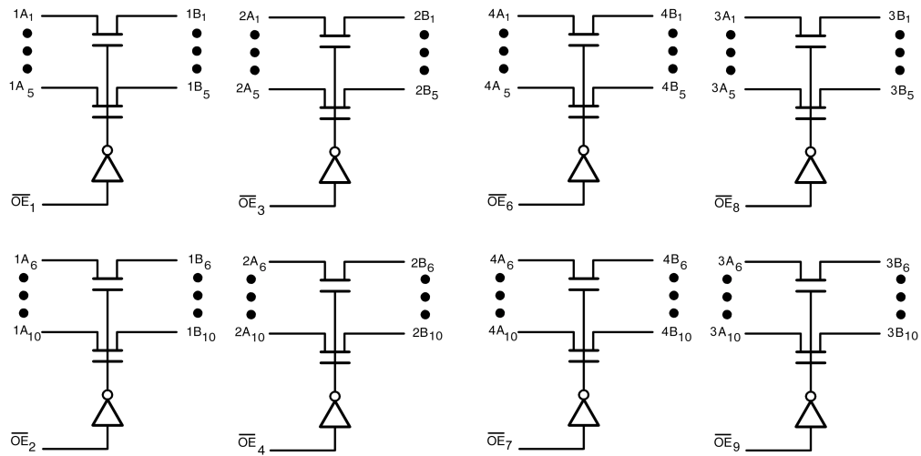
5-Bit Configuration
