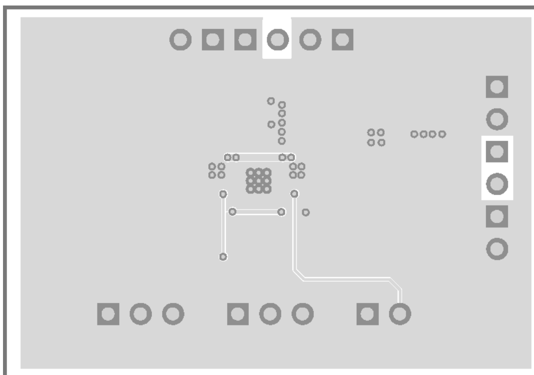
Figure 8. Bottom Layer
