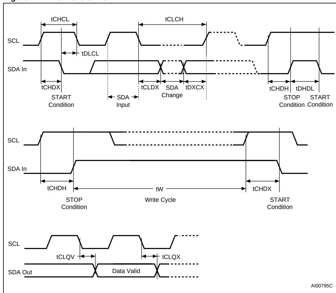
Figure 11. AC waveforms
