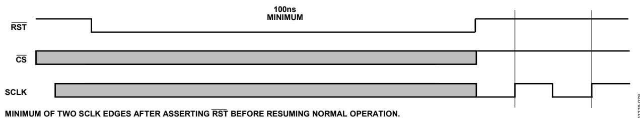
Figure 74. Reset Operation
