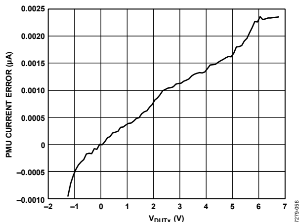
Figure 56. PMU FI Range E Output Current Error at -2\text{ μA} vs. Output Voltage; Output Voltage Is Pulled Externally
