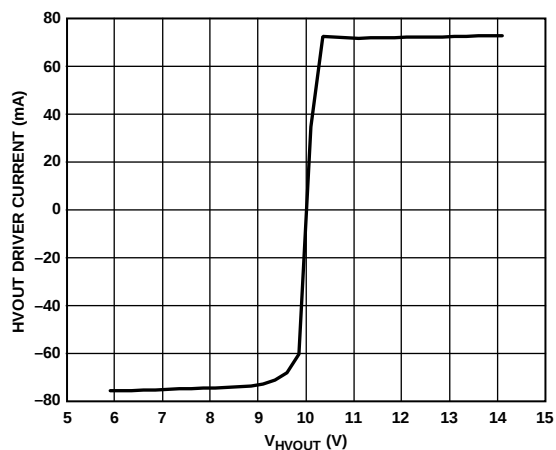
Figure 29. HVOOUT VHH Current Limit; V_{HH} = 10.0 V; V_{HVOOUT} Swept from -5.9 V to +14.1 V
