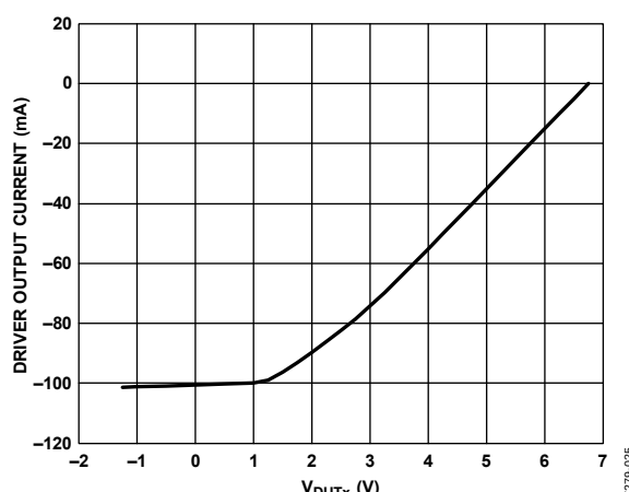
Figure 25. Driver Output Current Limit; Driver Programmed to 6.75 V; V_{DUTx} Swept from -1.25 V to +6.75 V
