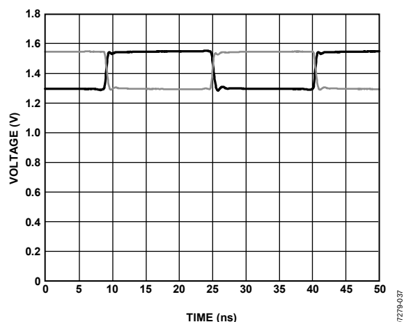
Figure 35. Comparator Output Waveform, COMP_QH0P, COMP_QH0N
