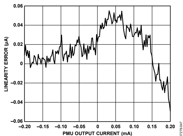
Figure 45. PMU Force Current Range C Linearity
