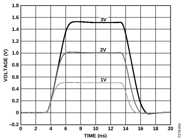
Figure 4. Driver Large Signal Response; V_H = 1.0\text{ V} , 2.0\text{ V} , 3.0\text{ V} ; V_L = 0.0\text{ V} ; 50\ \Omega Termination
