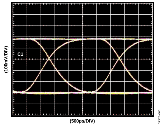
Figure 60. Eye Diagram, 400 Mbps, PRBS31; V_H = 1.0 V, V_L = 0.0 V
