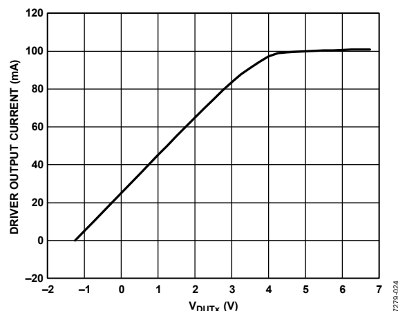
Figure 24. Driver Output Current Limit; Driver Programmed to -1.25 V; V_{DUTx} Swept from -1.25 V to +6.75 V
