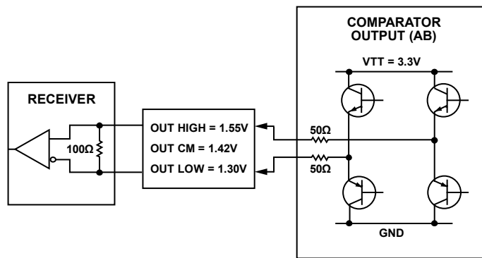
Figure 78. Comparator Output Scheme
