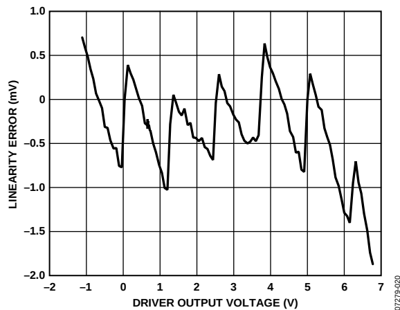
Figure 20. Driver V_H Linearity Error
