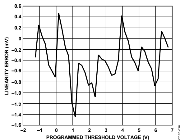
Figure 36. Comparator Threshold Linearity
