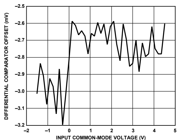
Figure 37. Differential Comparator CMRR
