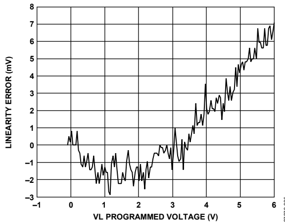
Figure 26. HVOUT VL Linearity Error
