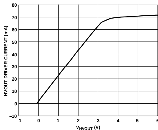
Figure 28. HVOOUT VH Current Limit; V_H = -0.1 V; V_{HVOOUT} Swept from -0.1 V to +6.0 V
