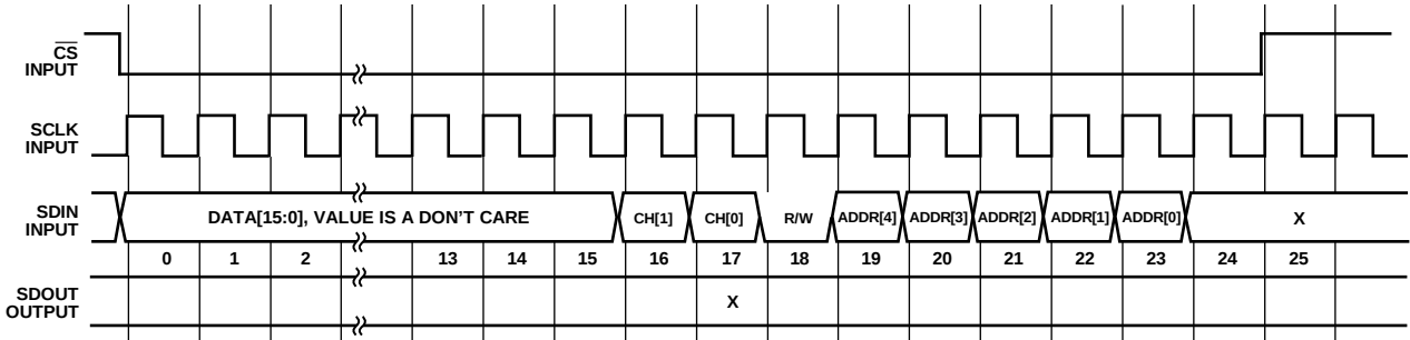
Figure 71. SPI Read Overview
