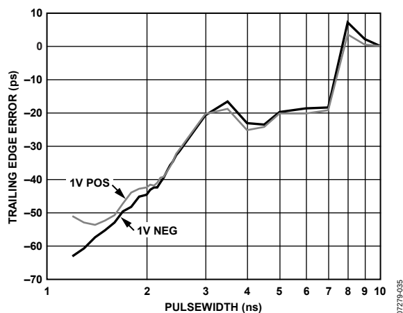
Figure 33. Comparator Minimum Pulse Width, 1.0 V
