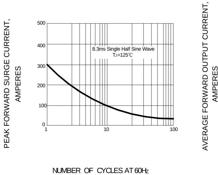
FIG.1 – PEAK FORWARD SURGE CURRENT
