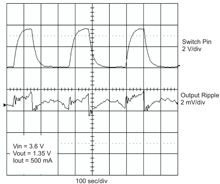
Figure 4. Output Ripple
